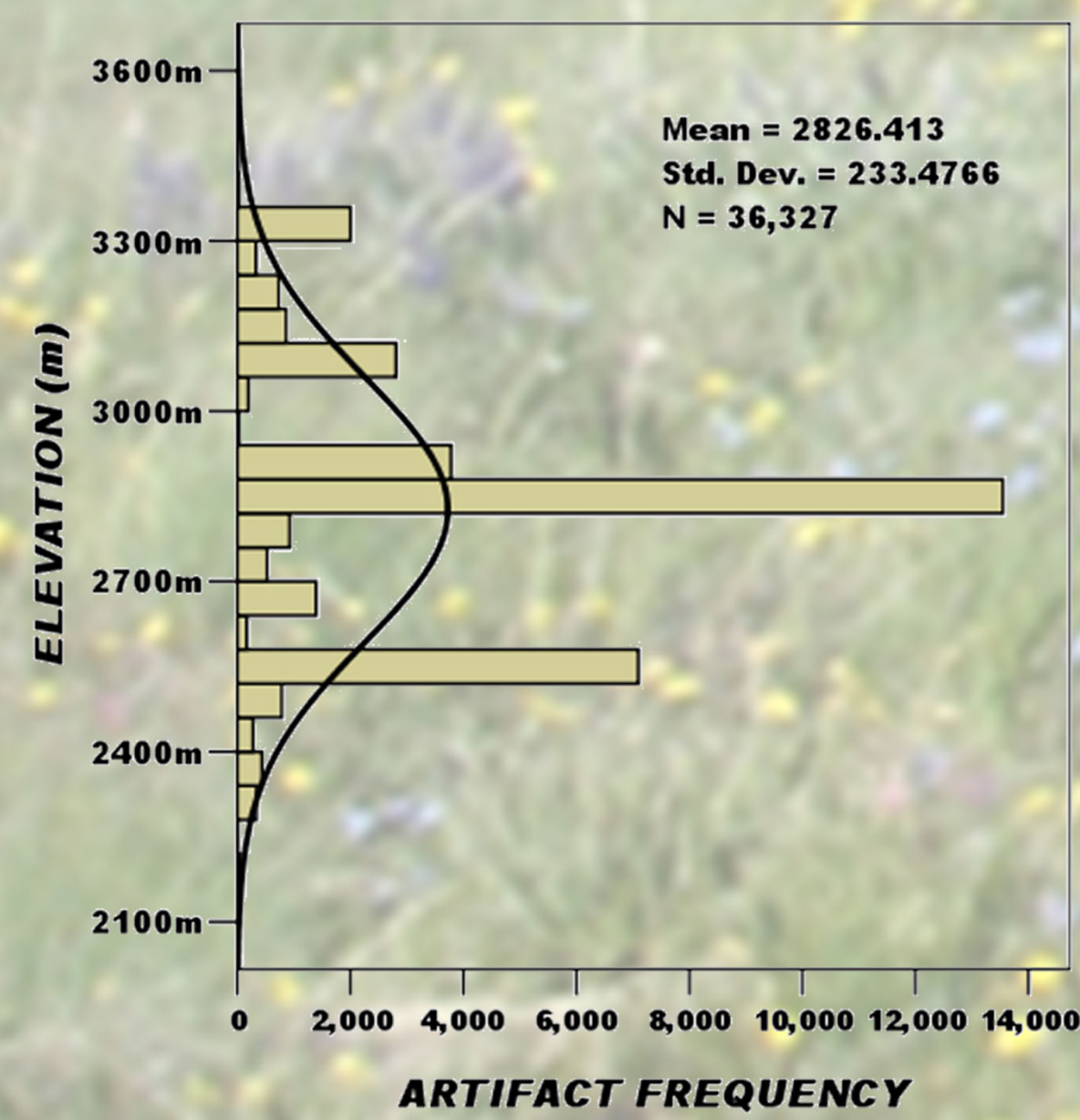
Figure 2. GRSLE Chipped Stone by Elevation
