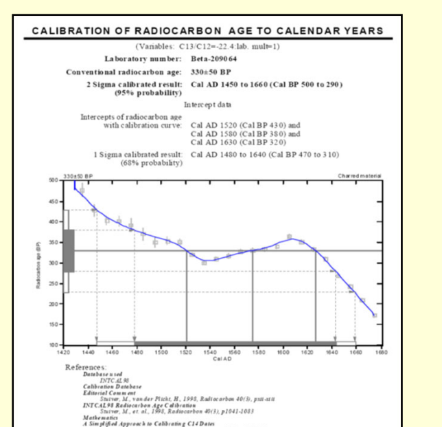
Figure 9: The radiocarbon age report for Tree Sample 1.
