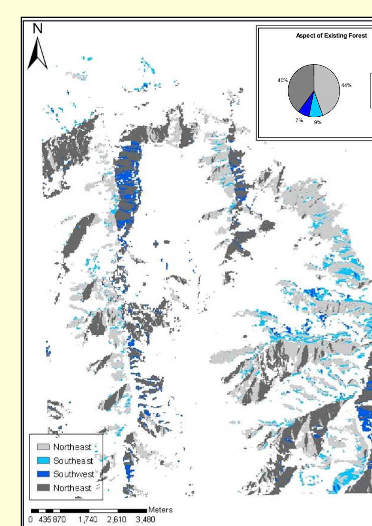
Figure 10: When forest cover and aspect are compared, a strong correlation is observed between forests and north-facing slopes
